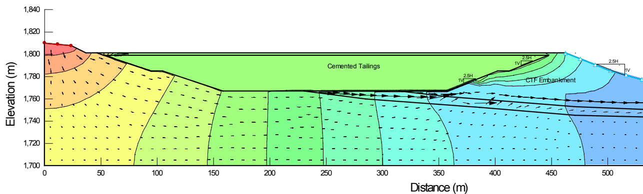
Figure 4-1 Groundwater Flow with Intact Lining System
